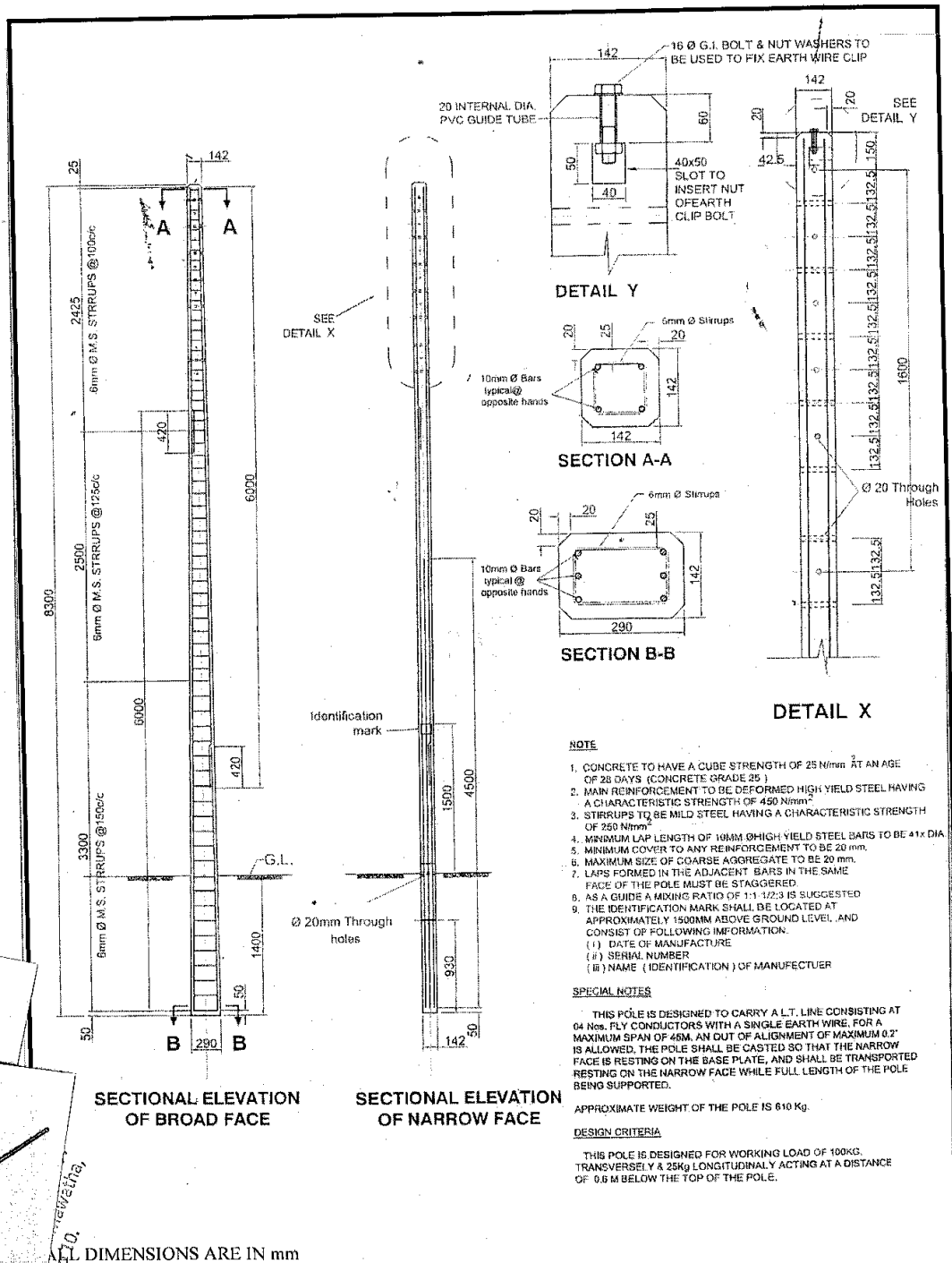
Figure: 8.3 m / 100 kg REINFORCED CONCRETE POLE
