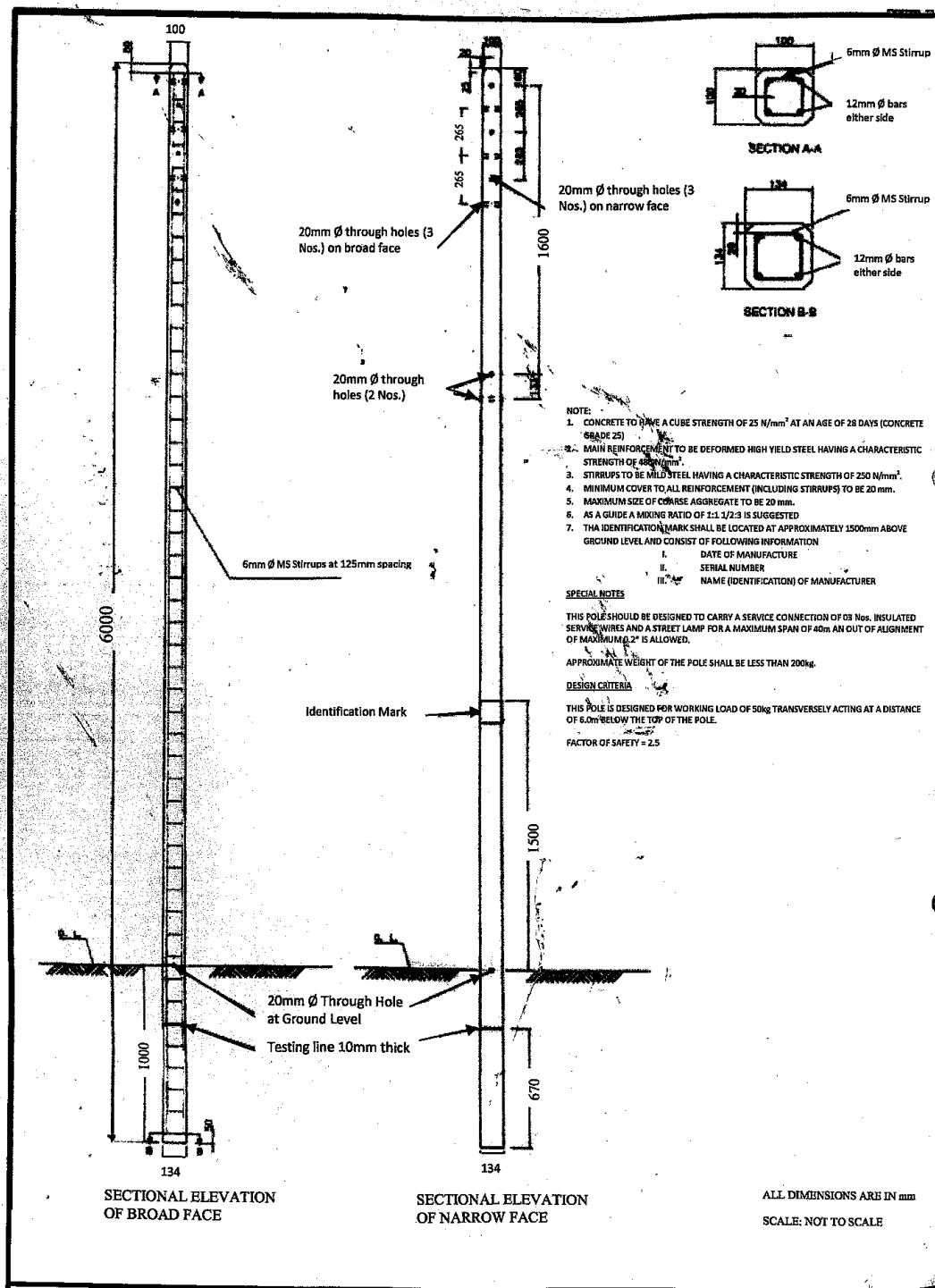
Figure: 6 m / 50 kg LIGHT WEIGHT REINFORCED CONCRETE POLE
