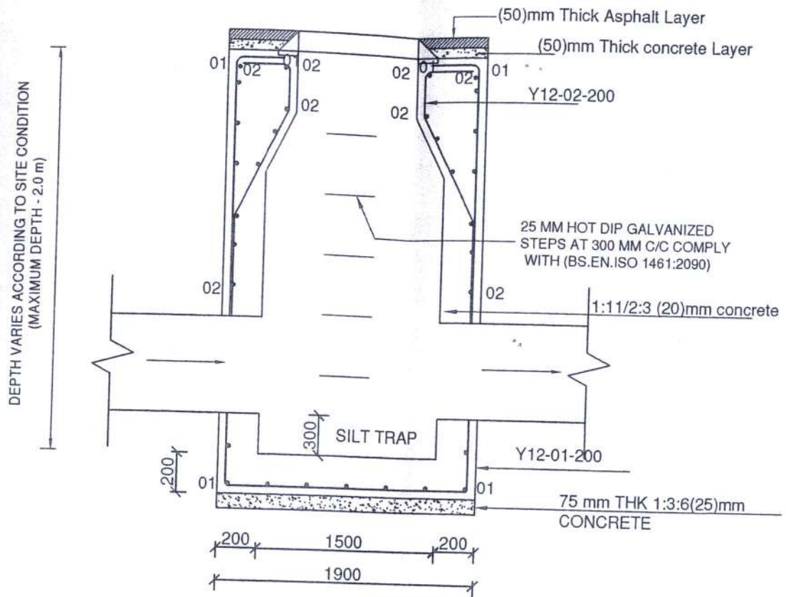
SECTION X-X
