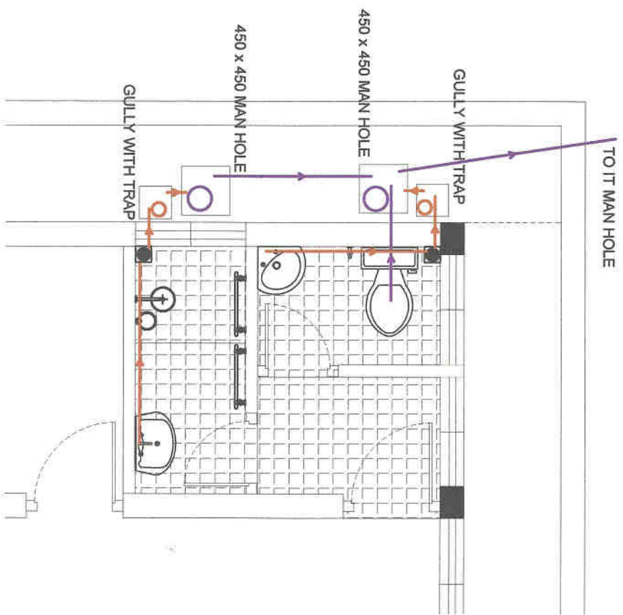
SEWERAGE AND WASTE WATER DISPOSAL SYSTEM
