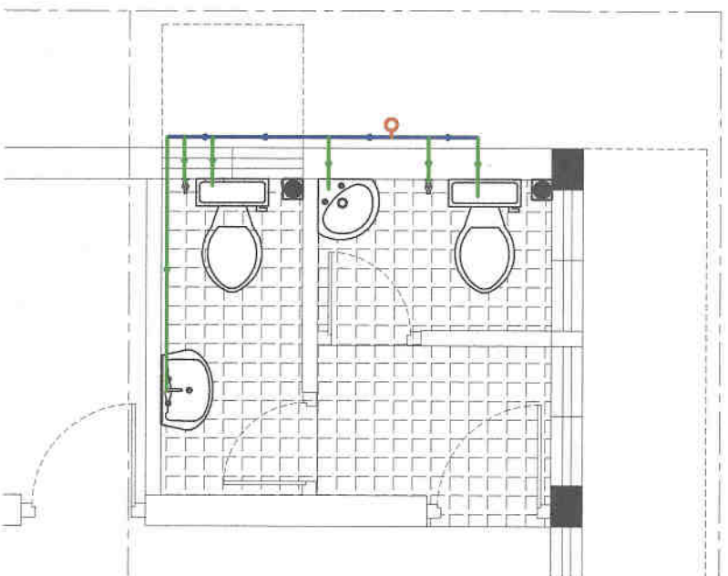
INTERNAL PLUMBING ARRANGEMENT - FIRST FLOOR
