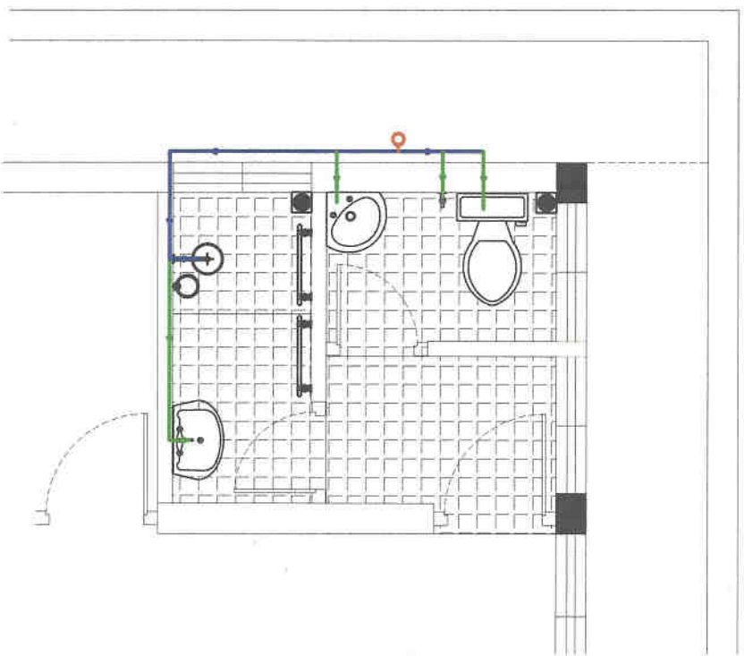
INTERNAL PLUMBING ARRANGEMENT - GROUND FLOOR
